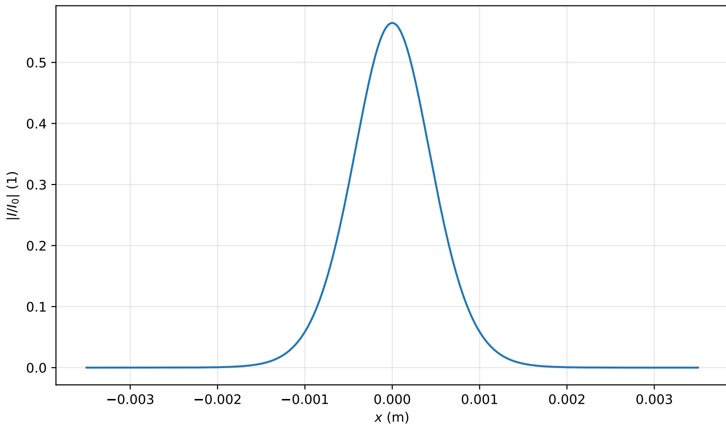
Intensity profile I(x, y = 0, z = 2.627m)/I_0 , P_{in}=0.4P_{cr} , artificial time
